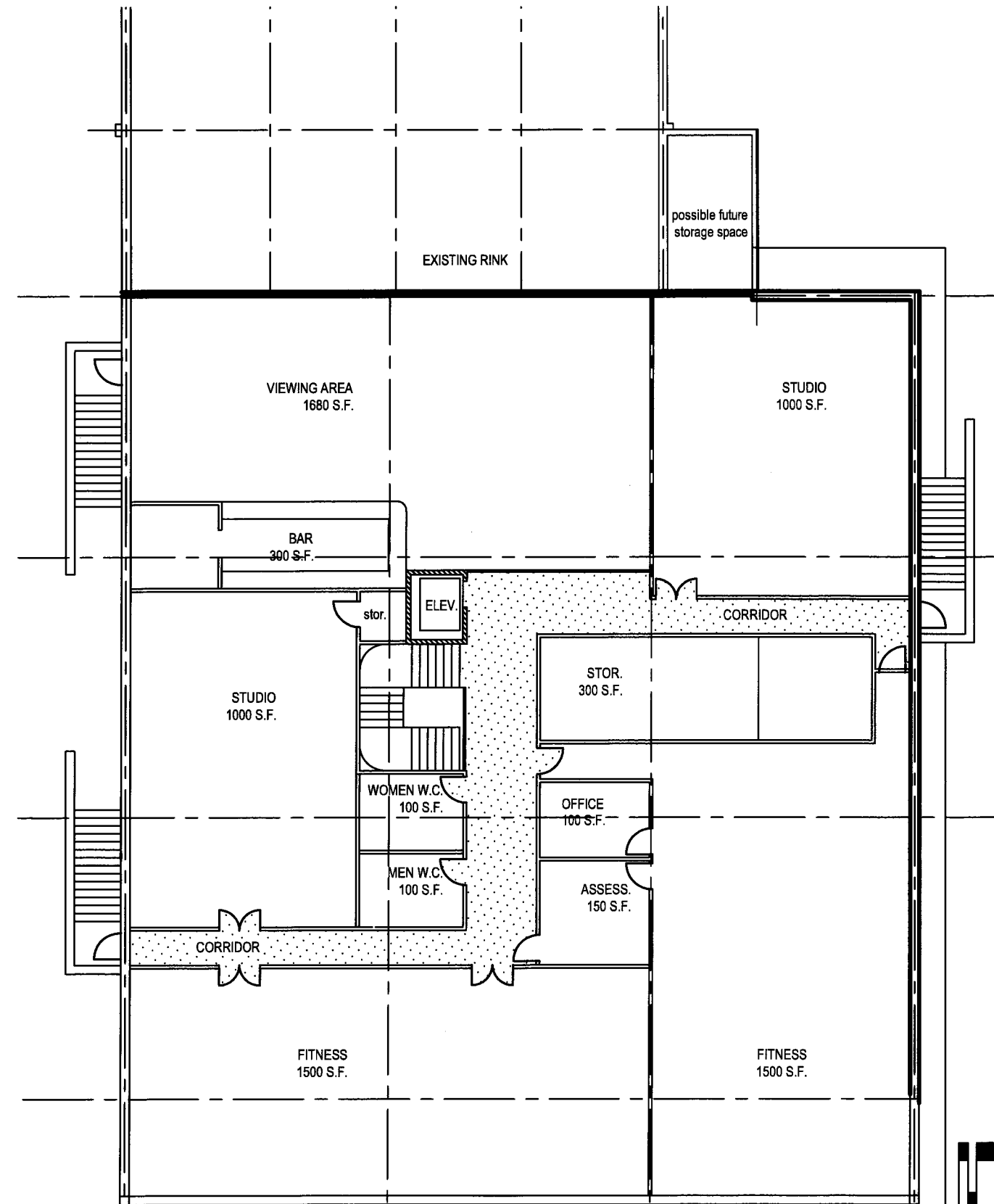
UPPER FLOOR PLAN- 9500 S.F.- option D
