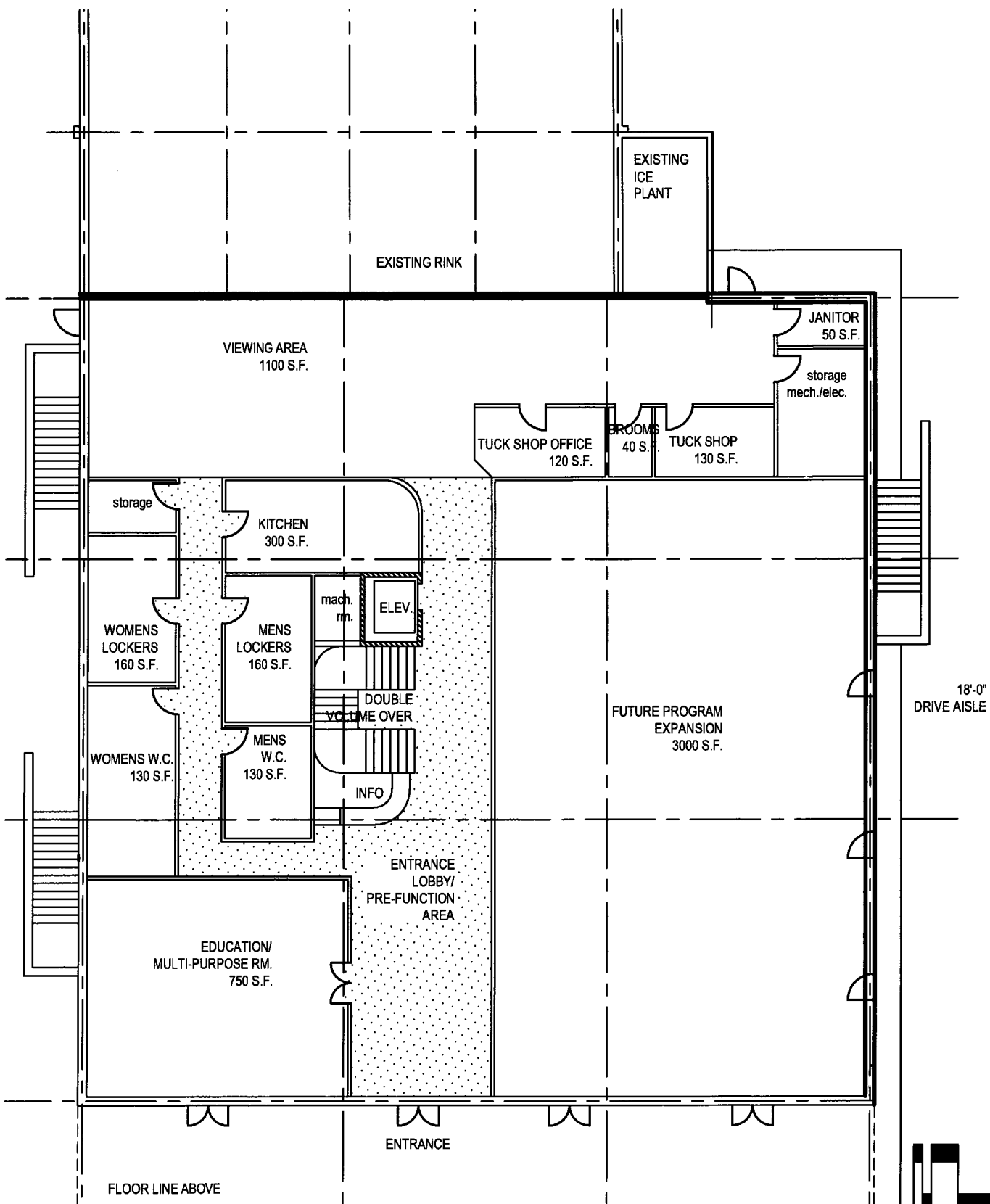
GROUND FLOOR PLAN-8500 S.F.- option D
